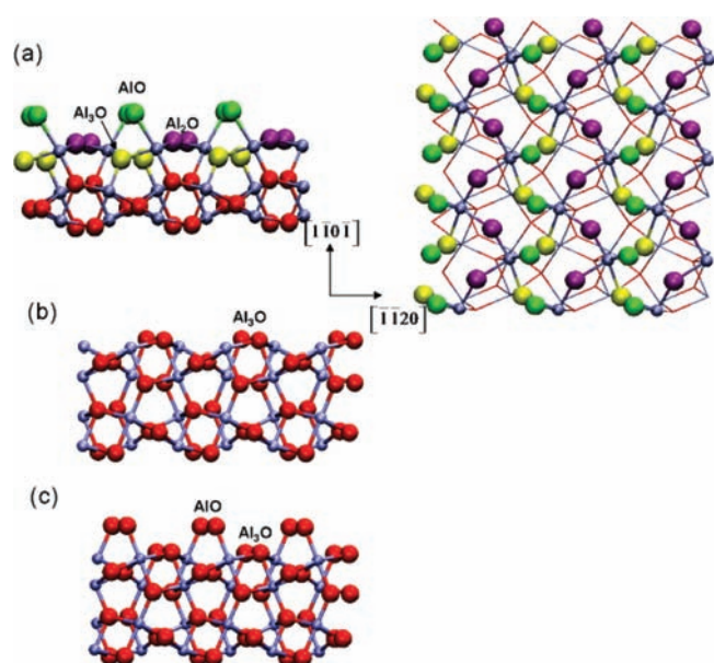
Figure 1. Surface structures of \alpha - \text{Al}_2\text{O}_3 ( 1\bar{1}02 ) obtained from (a) CTR measurement (side and top views of the structure are displayed on the left and right, respectively; the surface is terminated by equal numbers of singly (AlO, green), doubly (Al 2 O, purple), and triply (Al 3 O, yellow) coordinated oxygen atoms), (b) ideal bulk stoichiometric termination, and (c) X-ray reflectivity measurement. Red and blue spheres represent oxygen and aluminum, respectively.
